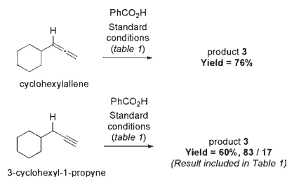
Scheme 3. Control Experiment with Cyclohexyllallene
